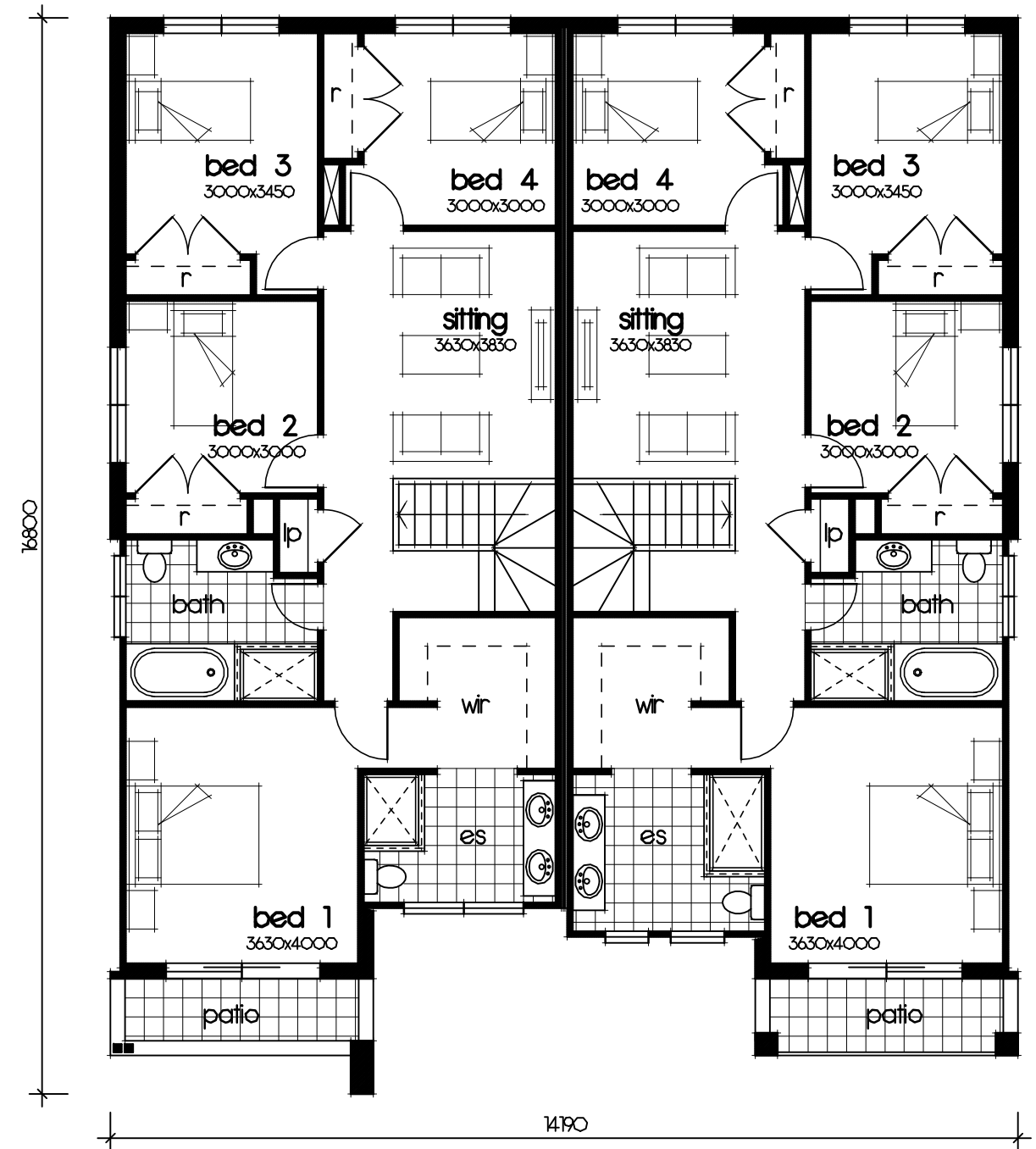
FIRST FLOOR PLAN JADE 25 - VOGUE FACADE
