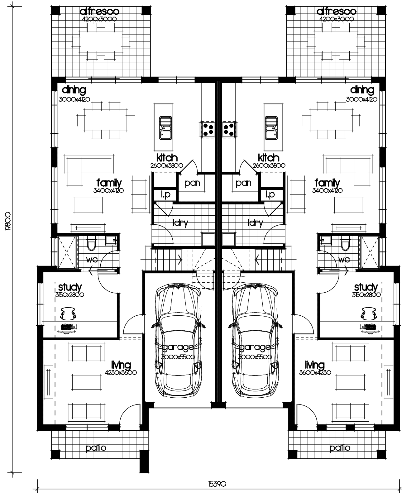
GROUND FLOOR PLAN JADE 25 - VOGUE FACADE
