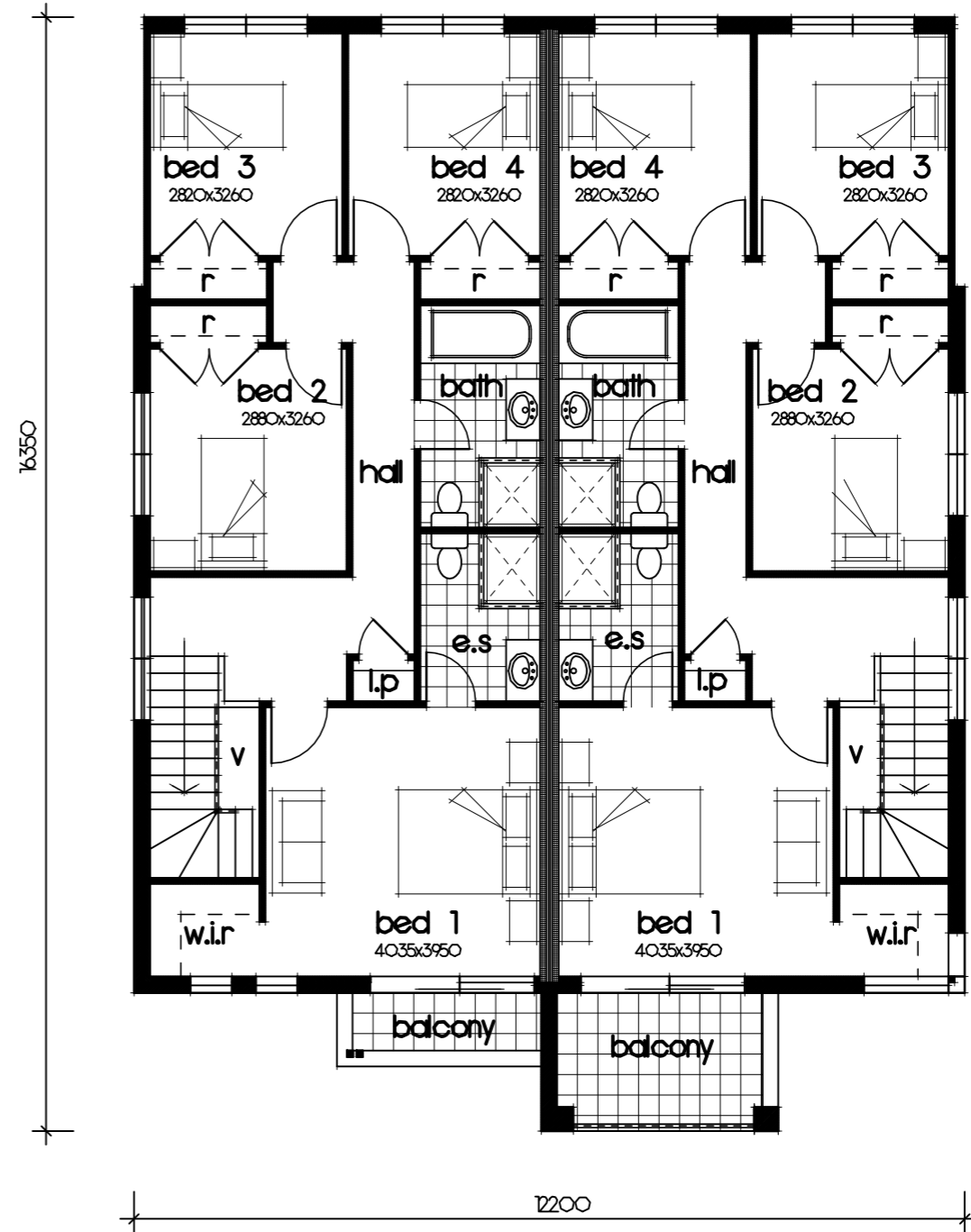
FIRST FLOOR PLAN BLOSSOM 21 - VOGUE FACADE
