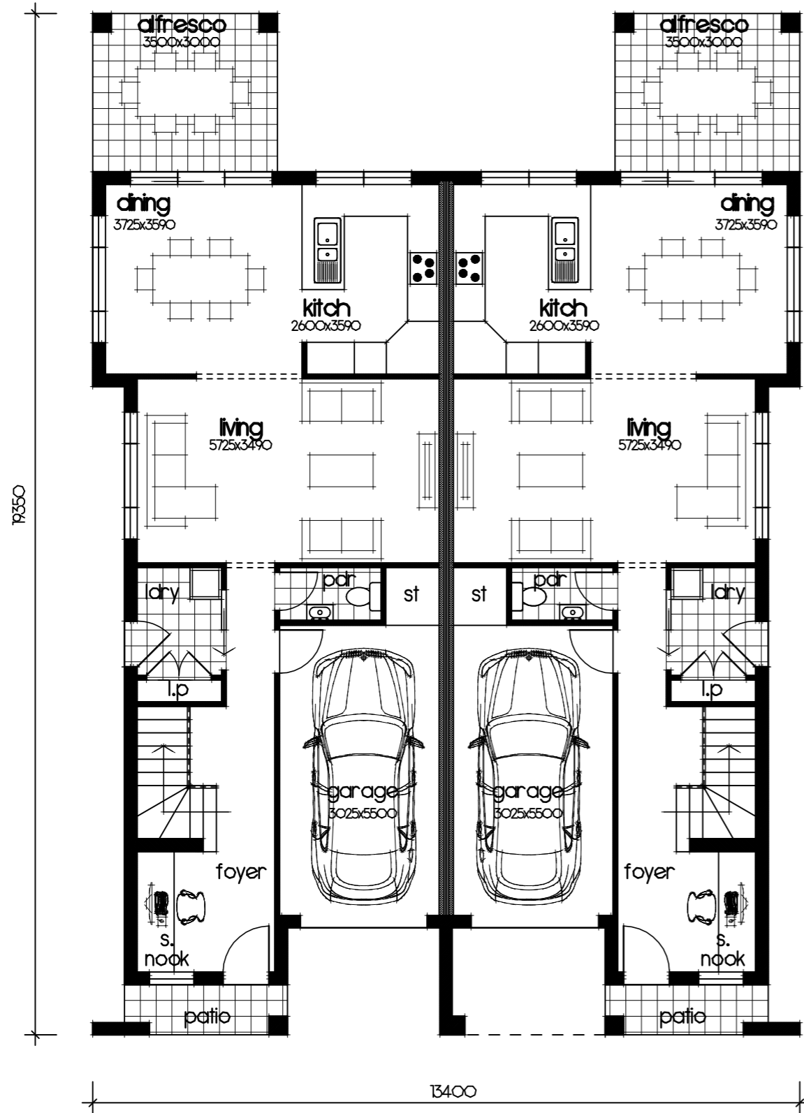
GROUND FLOOR PLAN BLOSSOM 21 - VOGUE FACADE
